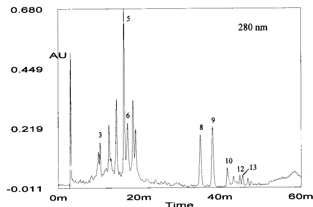
Figure 2. HPLC profile of apple puree phenolics obtained by Amberlite XAD-2 extraction: (3) (+)-catechin; (5) 5- O -caffeoylquinic acid; (6) (–)-epicatechin; (7) p -coumaric acid; (8) phloretin 2'-xylosylglucoside; (9) phloretin 2'-glucoside; (10) rutin; (12) quercetin 3-xyloside; (13) quercetin 3-rhamnoside.
