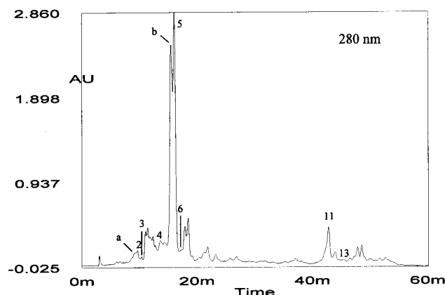
Figure 3. HPLC profile of pear puree phenolics obtained by Amberlite XAD-2 extraction: (a) 3- O -caffeoylquinic acid isomer; (2) 3- O -caffeoylquinic acid; (3) (+)-catechin; (4) p -hydroxybenzoic acid; (b) 5- O -caffeoylquinic acid isomer; (5) 5- O -caffeoylquinic acid; (6) (–)-epicatechin; (11) quercetin 3-galactoside; (13) quercetin 3-rhamnoside.
